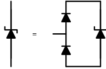
Figure 1. Pin Schematic
