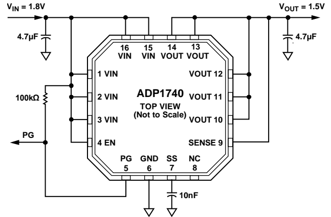
Figure 1. ADP1740 with Fixed Output Voltage, 1.5 V
