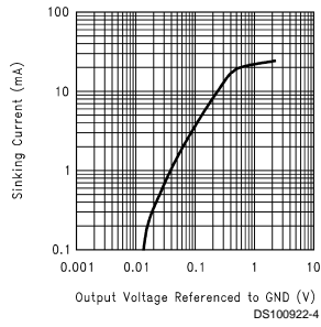
Sinking Current vs. Output Voltage ( V_S=2.2V )
