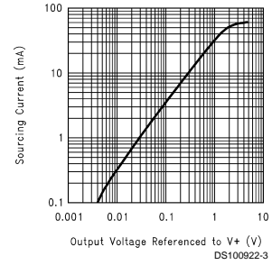
Sourcing Current vs. Output Voltage ( V_S=5V )
