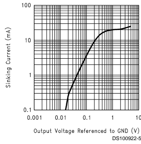
Sinking Current vs. Output Voltage ( V_S=5V )
