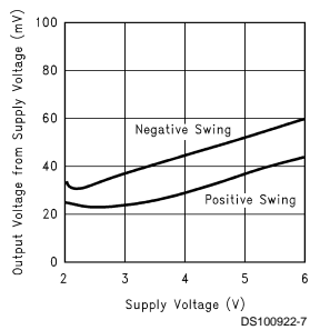
Output Voltage Swing vs. Supply Voltage ( R_L=2k\Omega )
