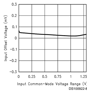
Input Offset Voltage vs. Input Common-Mode Voltage Range V_S=2.2V
