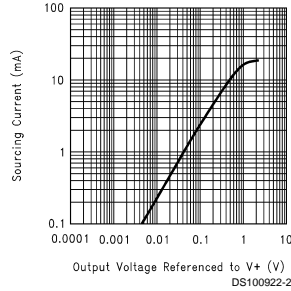
Sourcing Current vs. Output Voltage ( V_S=2.2V )
