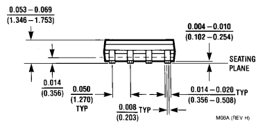
8-Pin Small Outline Order Number LMV722M or LMV722MX NS Package Number M08A
