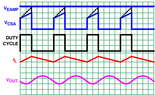
FIGURE 43. PWM OPERATION WAVEFORMS
