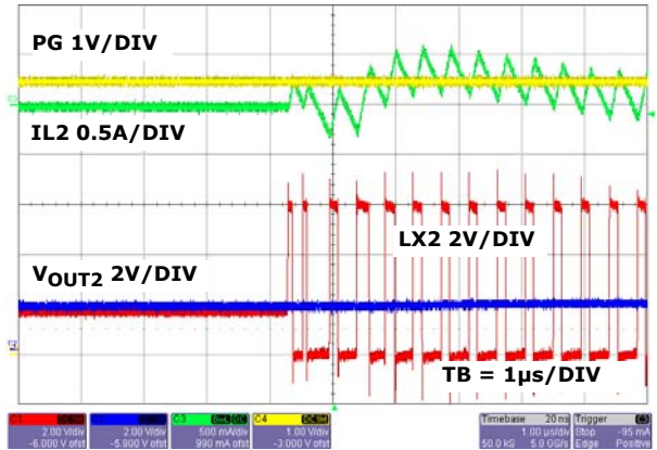
FIGURE 38. RECOVERY FROM HARD SHORT NEGATIVE CURRENT WAVEFORMS VOUT2 CHANNEL 2
