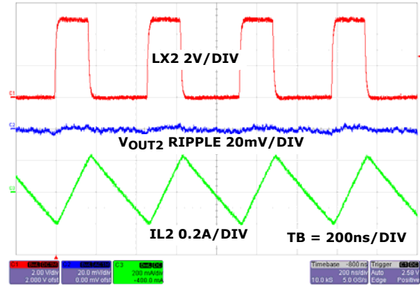
FIGURE 14. STEADY STATE OPERATION AT NO LOAD CHANNEL 2 (PWM)
