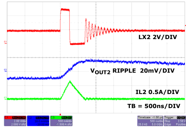
FIGURE 16. STEADY STATE OPERATION AT NO LOAD CHANNEL 2 (PFM)
