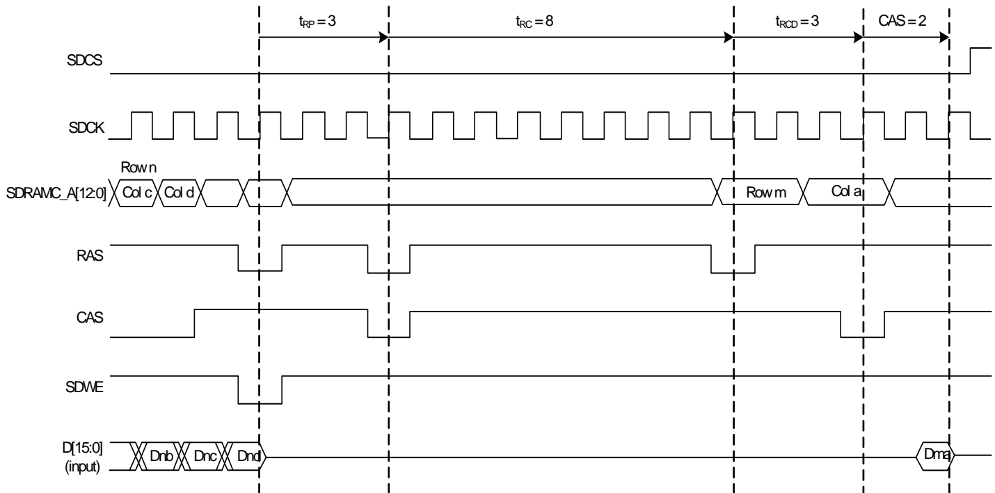
Figure 17-7. Refresh Cycle Followed by a Read Access
