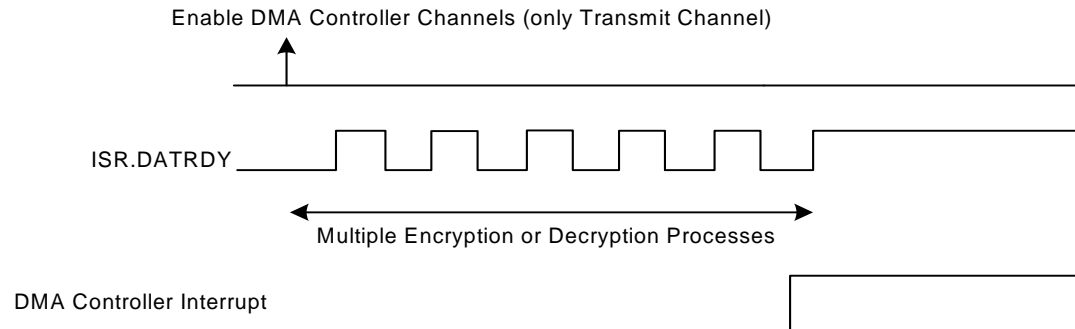
Figure 32-4. DMA Mode when MR.LOD is one
