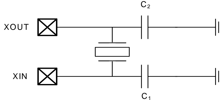
Figure 8-2. Oscillator Connections
