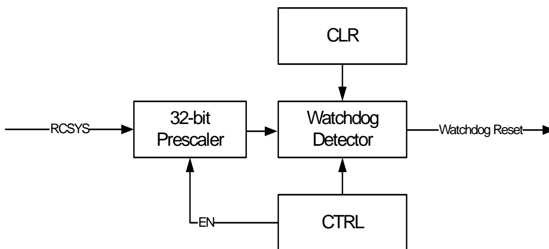
Figure 10-1. WDT Block Diagram
