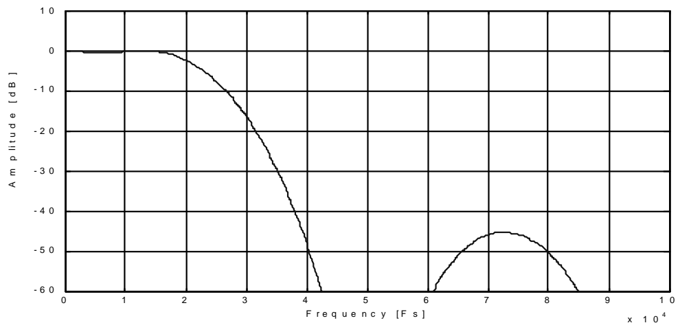
Figure 33-2. Frequency Response, EQ-FIR+COMB 4
