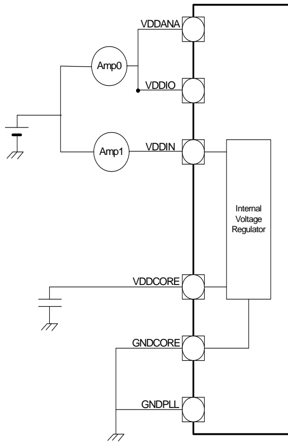
Figure 35-1. Measurement setup
