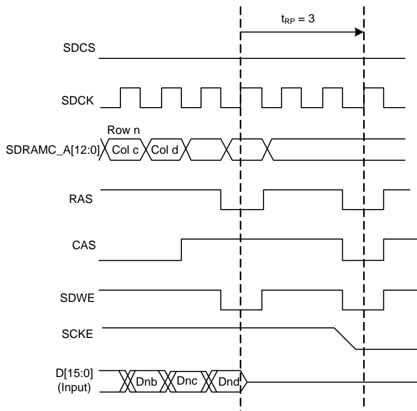
Figure 17-10. Deep Power-down Mode Behavior
