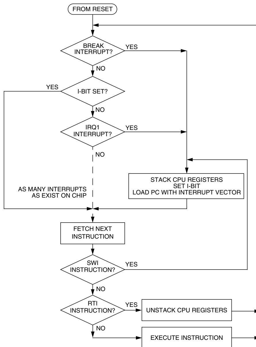
Figure 6-10. Interrupt Processing
