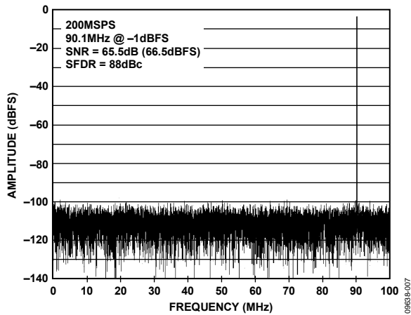
Figure 7. Single Tone FFT, f_{IN} = 90.1 MHz
