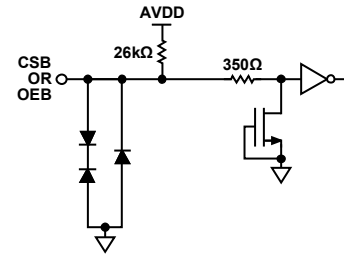
Figure 25. Equivalent CSB or OEB Input Circuit
