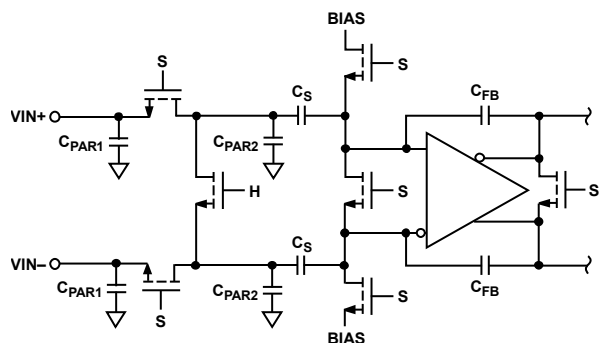
Figure 27. Switched Capacitor Input
