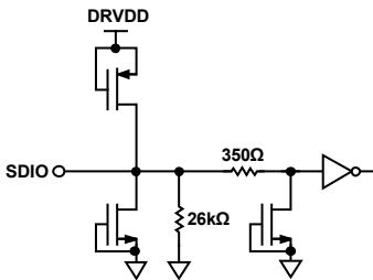
Figure 23. Equivalent SDIO Circuit
