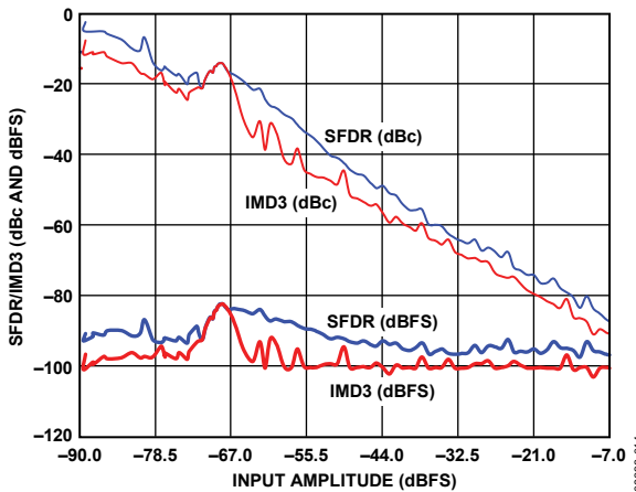
Figure 14. Two Tone SFDR/IMD3 vs. Input Amplitude ( A_{IN} ) with f_{IN1} = 89.12 MHz, f_{IN2} = 92.12 MHz
