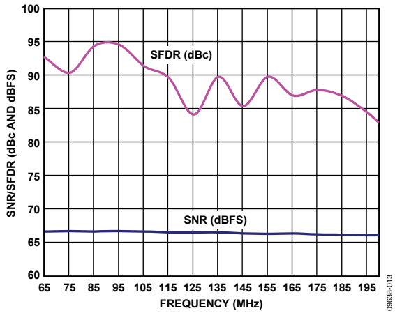
Figure 13. Single Tone SNR/SFDR vs. Input Frequency ( f_{IN} )
