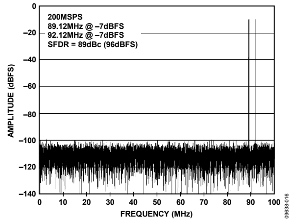
Figure 16. Two Tone FFT with f_{IN1} = 89.12 MHz, f_{IN2} = 92.12 MHz
