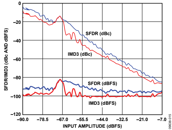
Figure 15. Two Tone SFDR/IMD3 vs. Input Amplitude ( A_{IN} ) with f_{IN1} = 184.12 MHz, f_{IN2} = 187.12 MHz
