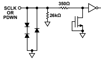
Figure 24. Equivalent SCLK or PDWN Input Circuit
