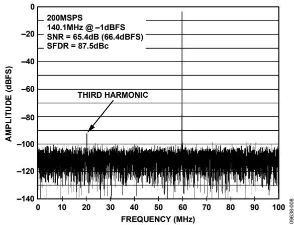
Figure 8. Single Tone FFT, f_{IN} = 140.1 MHz
