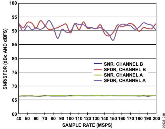
Figure 18. Single Tone SNR/SFDR vs. Sample Rate ( f_s ) with f_{IN} = 90.1 MHz
