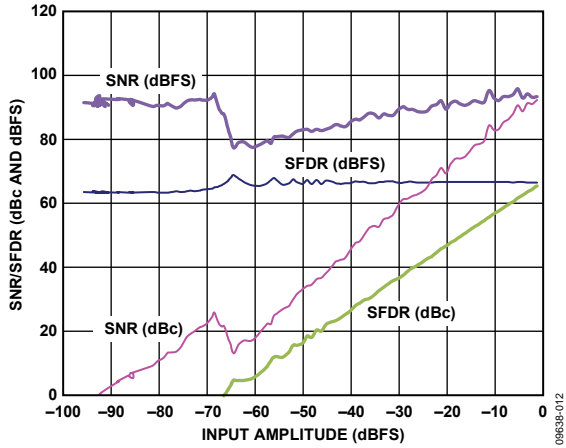
Figure 12. Single Tone SNR/SFDR vs. Input Amplitude ( A_{IN} ), f_{IN} = 90.1 MHz
