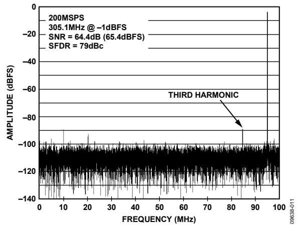
Figure 11. Single Tone FFT, f_{IN} = 305.1 MHz
