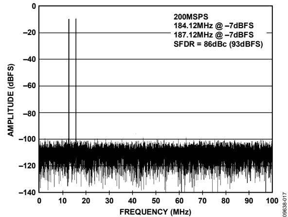
Figure 17. Two Tone FFT with f_{IN1} = 184.12 MHz, f_{IN2} = 187.12 MHz
