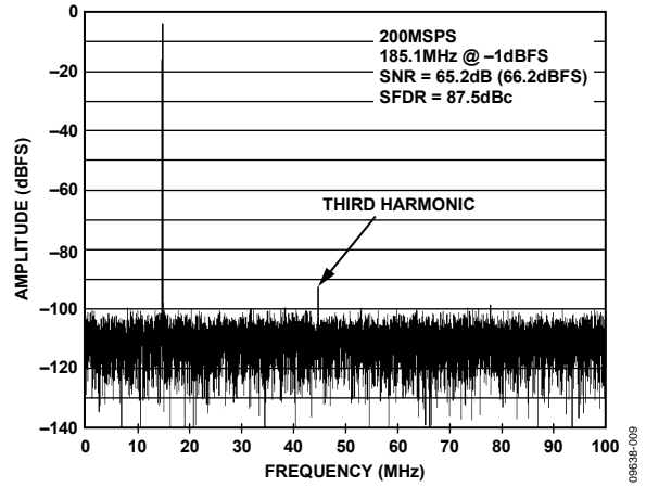
Figure 9. Single Tone FFT, f_{IN} = 185.1 MHz
