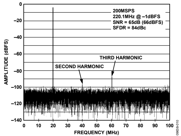
Figure 10. Single Tone FFT, f_{IN} = 220.1 MHz
