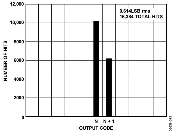
Figure 19. Grounded Input Histogram
