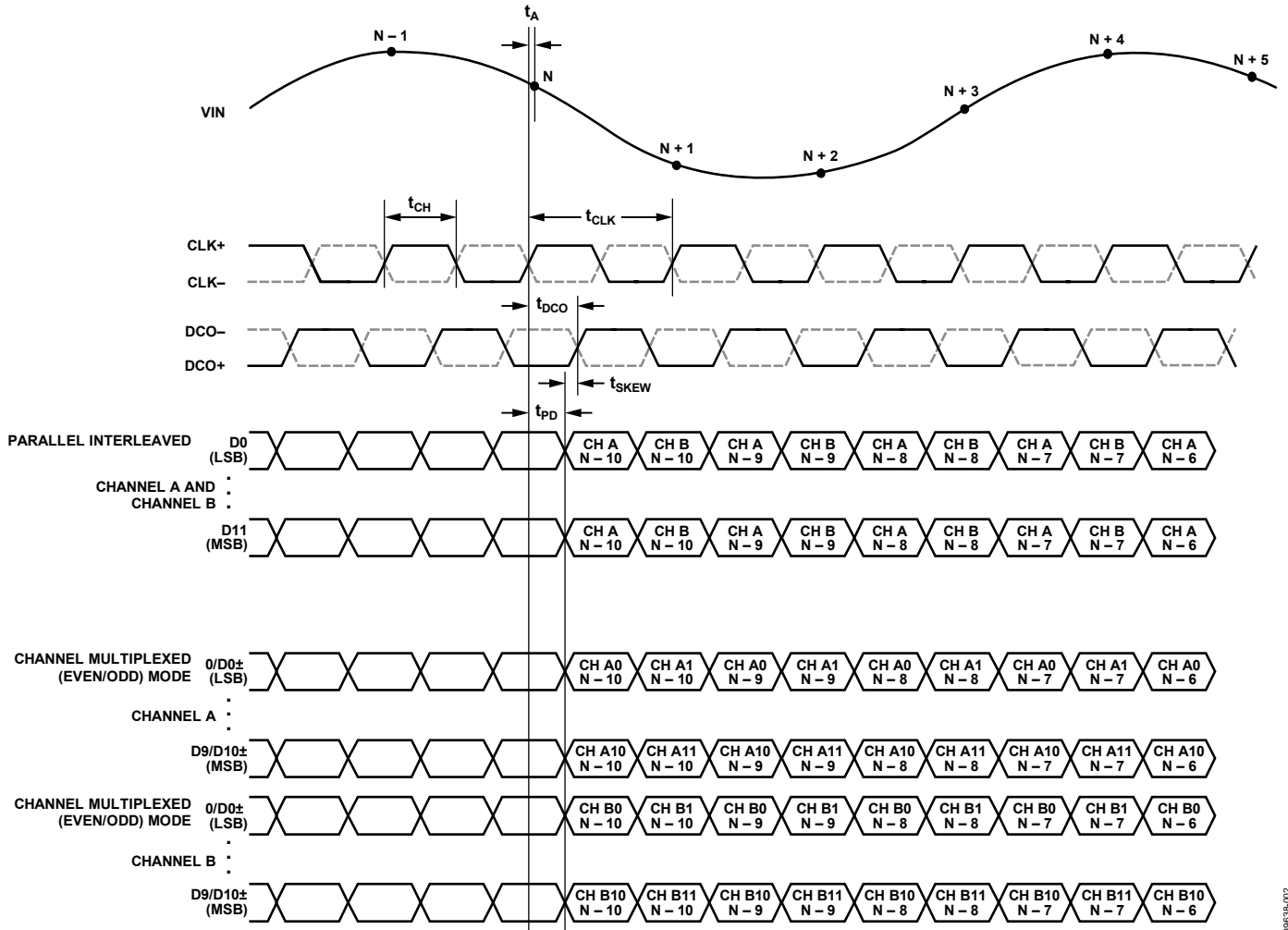
Figure 2. LVDS Modes for Data Output Timing Latency, NSR Disabled (Enabling NSR Adds an Additional Three Clock Cycles of Latency)
