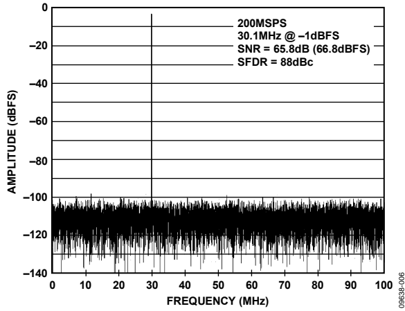
Figure 6. Single Tone FFT, f_{IN} = 30.1 MHz
