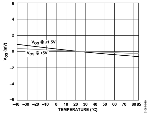
Figure 10. V_{OS} vs. Temperature
