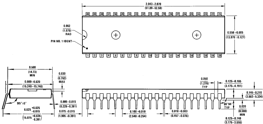
Molded Dual-In-Line Package (N) Order Number MM5486 NS Package Number N40A
