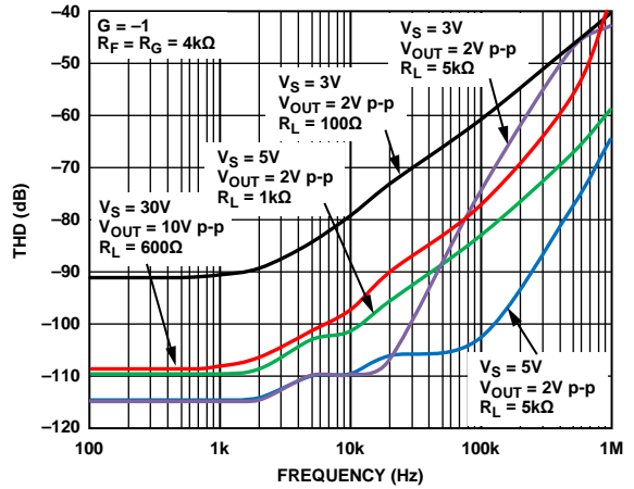
Figure 16. Total Harmonic Distortion vs. Frequency
