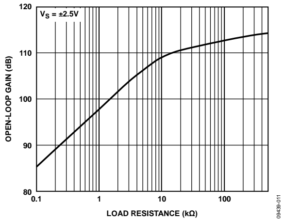
Figure 14. Open-Loop Gain vs. Load Resistance
