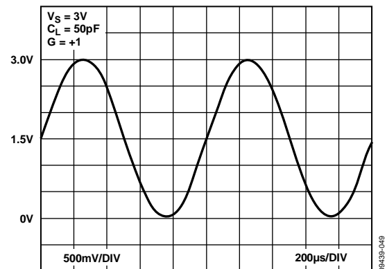
Figure 3. Output Swing, +V_S = +3\text{ V} , G = +1
