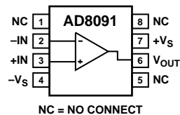
Figure 1. SOIC-8 (R-8)
