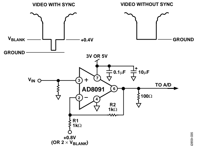
Figure 35. Sync Stripper
