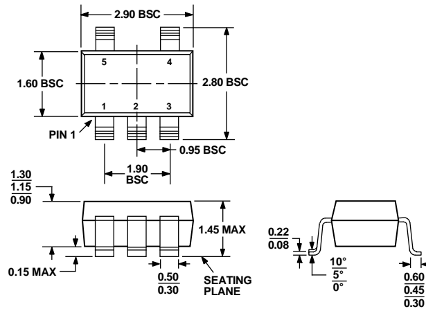
Figure 39. 5-Lead Small Outline Transistor Package [SOT-23] (RT-5) Dimensions shown in millimeters
