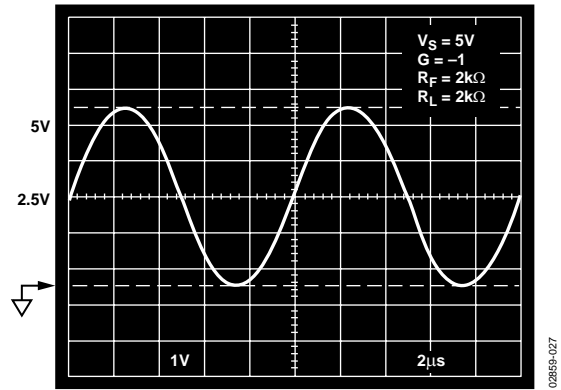
Figure 27. Output Swing; G = -1 , R_L = 2k\Omega
