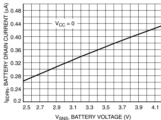
Battery Drain Current versus Battery Voltage
