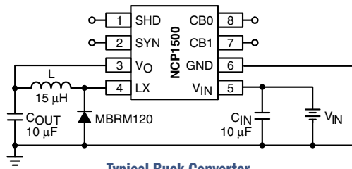
Typical Buck Converter
