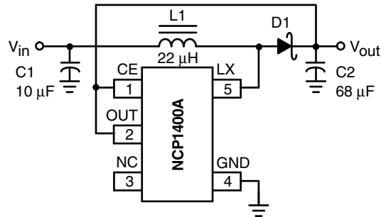
Typical Boost Converter
