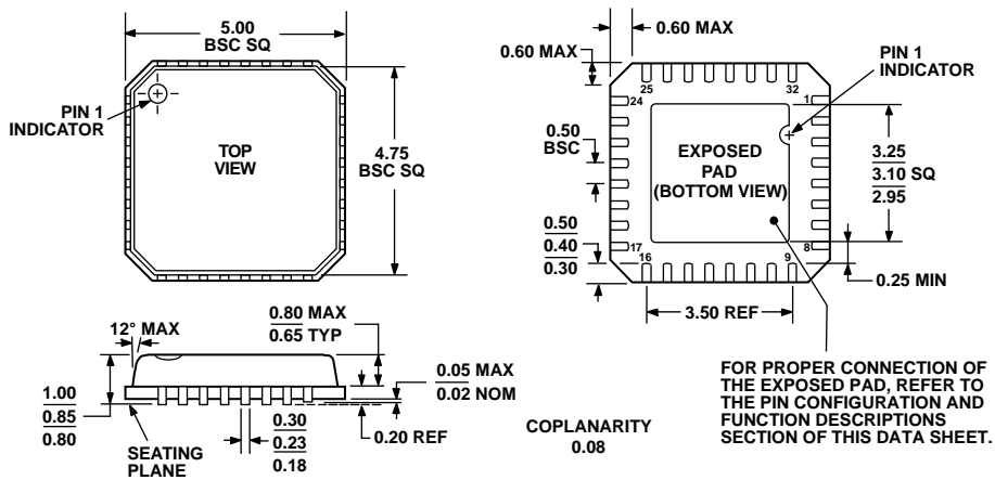
COMPLIANT TO JEDEC STANDARDS MO-220-VHHD-2 Figure 52. 32-Lead Lead Frame Chip Scale Package [LFCSP_VQ] 5 mm × 5 mm Body, Very Thin Quad (CP-32-2) Dimensions shown in millimeters
